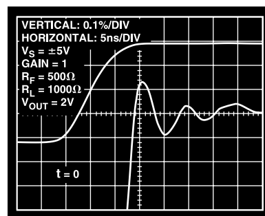
Figure 18. Settling Time
